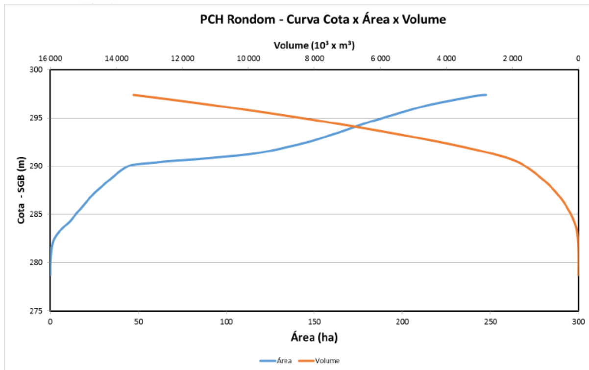
Figura 32 – PCH Rondon – Curva CAV
