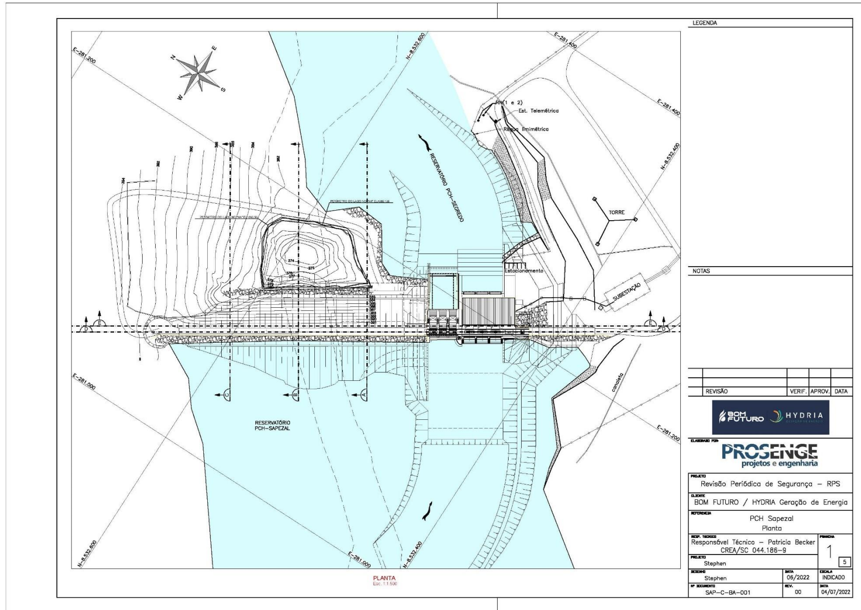
Figura 9 – Arranjo Geral – RPS
